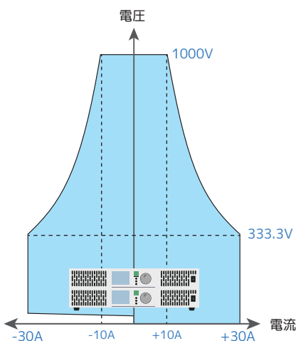
PBW-103HS動作範囲
